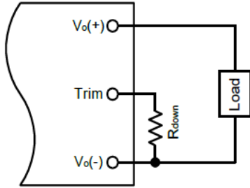
Figure 15. Circuit to Decrease Output Voltage
