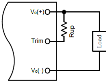
Figure 16. Circuit to Increase Output Voltage
