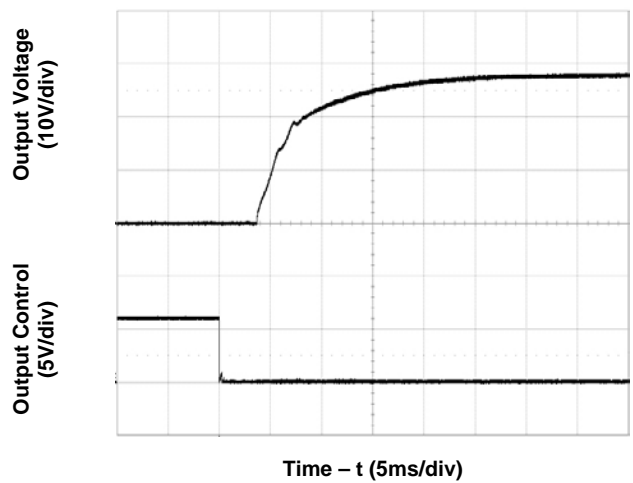
Figure 6. Start-Up from Enable Control (typical Vin, zero load, 470µF external output capacitance)
