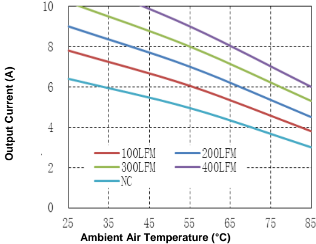
Figure 9. Current Derating Curve for Airflow Direction 3 (Ref. Fig. 11 for Airflow Direction; typical V_{in} , open frame, unit soldered onto test fixture board)
