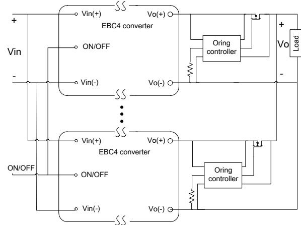
Figure 17. The connection diagram of parallel version EBC4 converters with ORing devices
