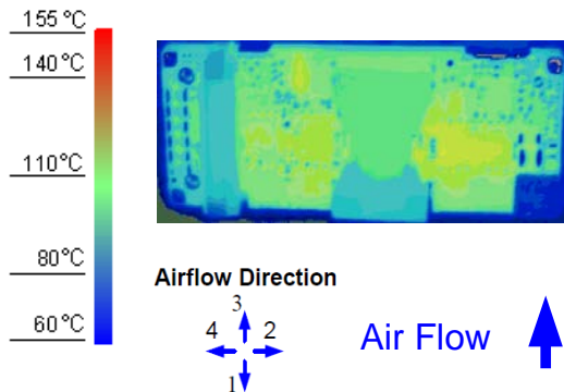
Figure 11. Thermal Image for Airflow Direction 3 (7A output, 55^{\circ}C ambient, 200 LFM, typical V_{in} , unit soldered onto a fixture board)
