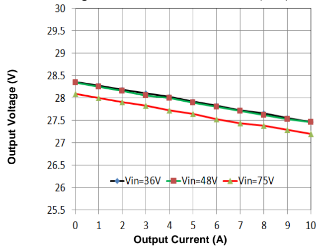
Figure 4. Output Droop Characteristic (parallel version)
