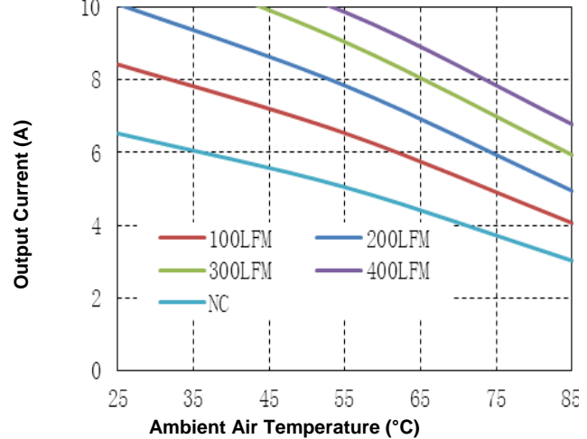
Figure 10. Current Derating Curve for Airflow Direction 3 (Ref. Fig. 11 for Airflow Direction; typical V_{in} , baseplate, unit soldered onto test fixture board)
